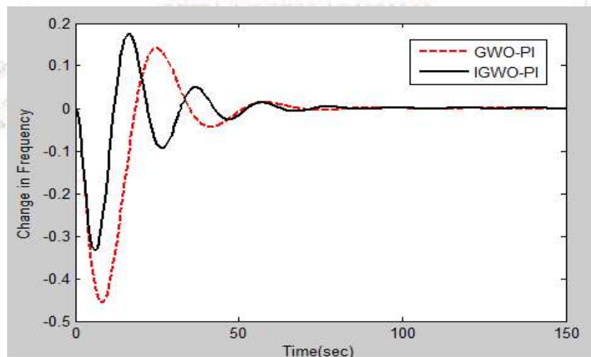
Fig 5: Comparative Frequency Deviations of controllers under case-1
