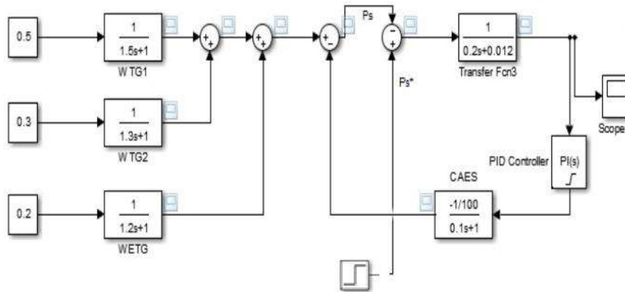
Fig 2: Simulation Block diagram of Proposed System
