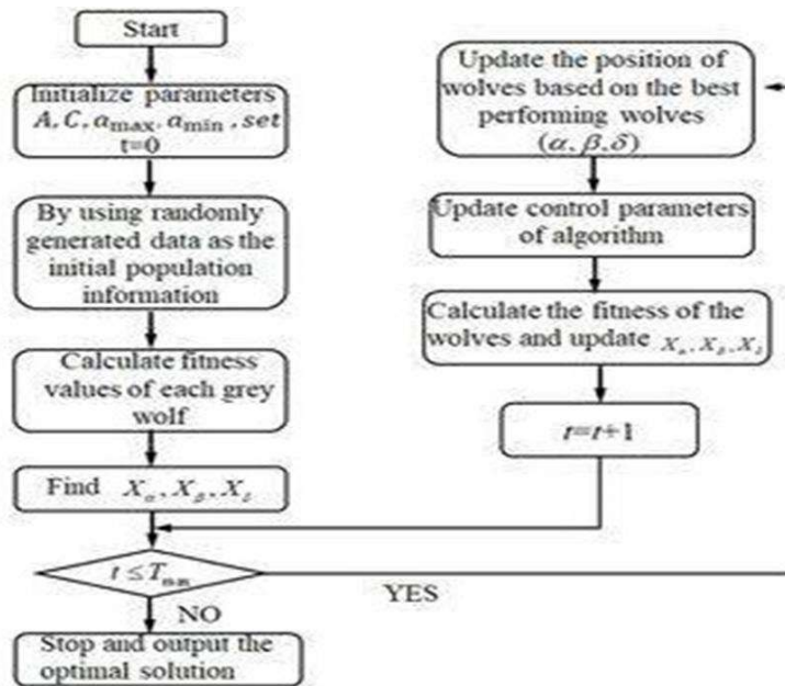
Fig 4: Flowchart of IGWO technique
