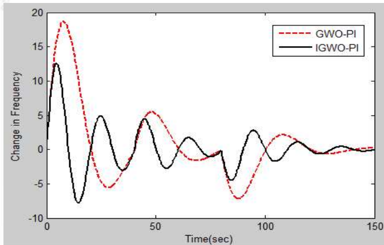
Fig 7: Comparative Frequency Deviations of controllers under case-2
